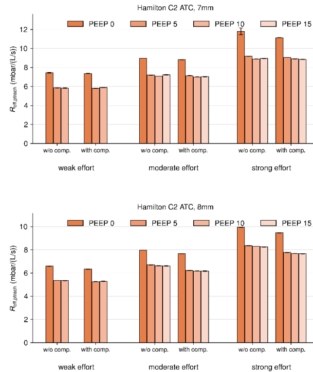
Fig. SI 2: Effect of flow sensor placement on effective tracheal resistance. In the standard measurement configuration, the thermal mass flow sensor and airway pressure adapter are placed between the flexible tube and the Y-piece. The Hamilton C2 (and C6) ventilators provide their own flow sensor and airway pressure adapter, which is placed between the Y-piece and our airway pressure adapter. This corresponds to the standard measurement configuration, in which the resistance of our thermal mass flow sensor and airway pressure adapter is not compensated by the demand-flow control of the ventilator and thus adds to the total resistance of the respiratory system. However, by placing the Hamilton flow and pressure sensor adapter between the flexible tube and our thermal mass flow sensor and airway pressure adapter, the resistance of the latter can be compensated by the ventilator. Comparison of effective tracheal resistance without flow sensor resistance compensation (left bars) and with flow sensor resistance compensation (right bars) shows only negligible effects, except at strong respiratory effort where flow sensor resistance compensation lowers R_{eff,ptach} by up to 0.5 mbar/(L/s).
