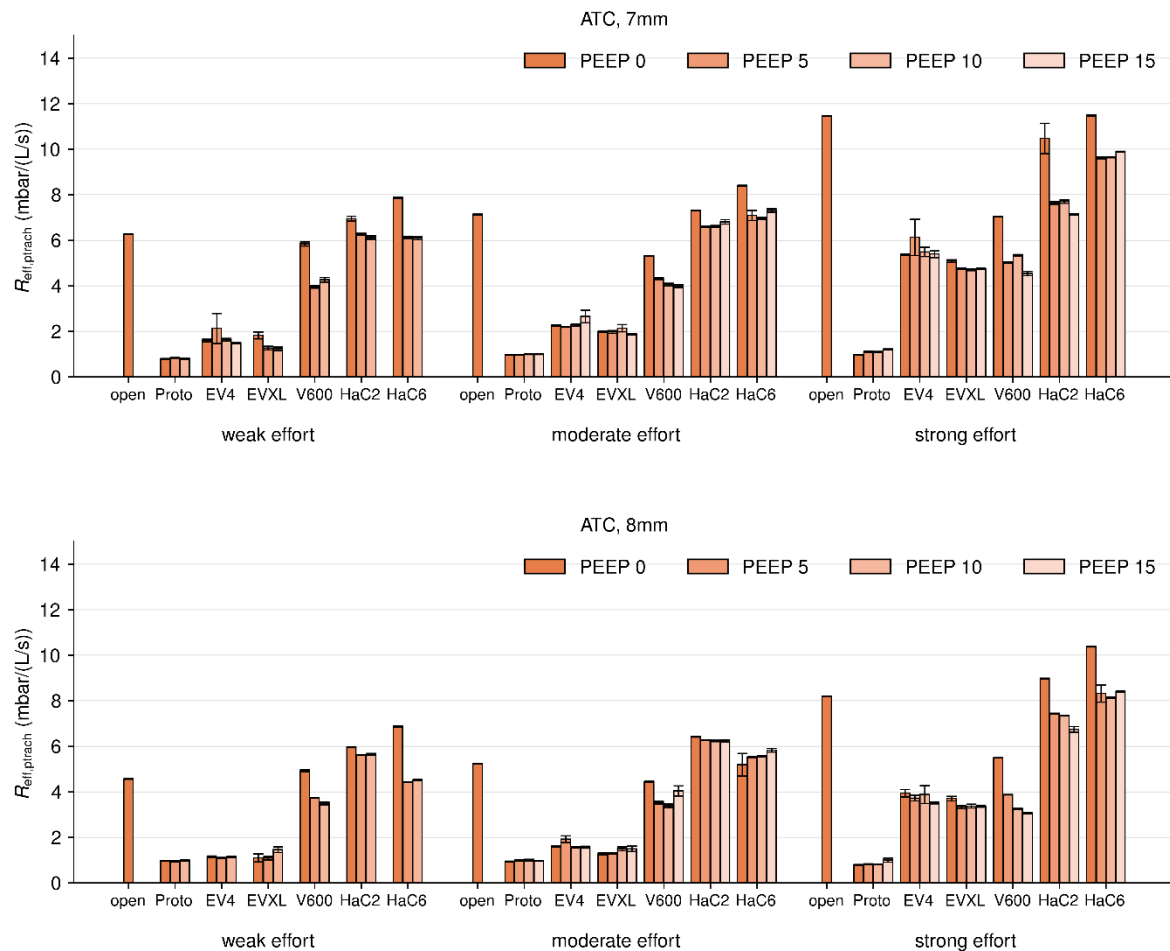
Fig. SI 1: Effective tracheal resistance during ATC during inspiration. Effective tracheal resistance R_{eff,ptrach,in} in inspiration (positive flow) during ATC with a 7 mm (top) and 8 mm (bottom) endotracheal tube, shown for weak, moderate, and strong inspiratory effort, different PEEP levels, and all tested ventilators. R_{eff,ptrach,in} is computed during the positive flow phase as the mean absolute difference between the tracheal pressure and PEEP, divided by the mean inspiratory flow. PEEP is the end-expiratory tracheal pressure of the current breathing cycle, measured as the mean tracheal pressure between 80 ms and 40 ms before the start of the next inspiration.
