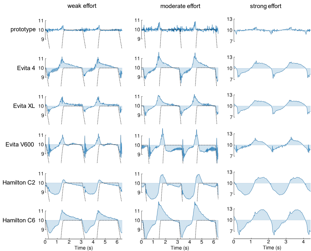
Fig. 1: Airway pressure control during CPAP. Representative airway-pressure recordings (in mbar) during simulated spontaneous breathing through a 7 mm endotracheal tube at PEEP = 10 mbar. Columns show weak, moderate, and strong inspiratory effort. Rows show the tested ventilators. Airway pressure (blue) is plotted as deviation from the set PEEP level during two consecutive breathing cycles; the horizontal line marks zero deviation. In an ideal CPAP system, airway pressure would remain on this line throughout the breathing cycle. The dotted line shows P_{mus} + PEEP and marks the timing of inspiration and expiration. The P_{mus} trace is truncated to keep the pressure deviations visible; the full, untruncated P_{mus} trace is shown in Fig. 3. Commercial ventilators showed substantial flow-dependent pressure deviations that increased with respiratory effort.
